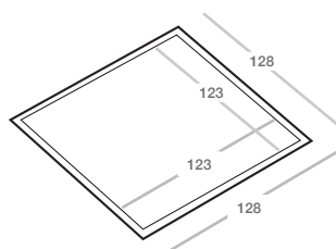
Phleximax grating for tiled floor
